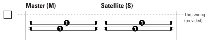
Continuous Row with Master/Satellite, 2 Lamps, 1cct.
