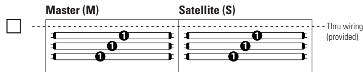
Continuous Row with Master/Satellite, 3 Lamps, 1cct.
