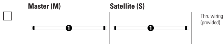
Continuous Row with Master/Satellite, 1 Lamp, 1cct.
